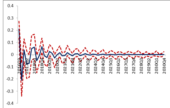
Figure 14. n/o Growth (10% b/expenditure shock)
