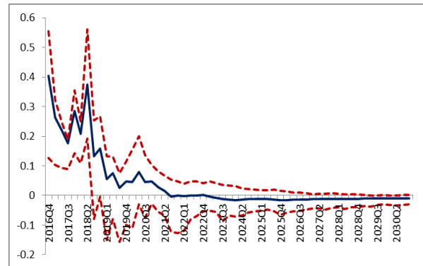
Figure 18. Imports (10% o/prod shock)
